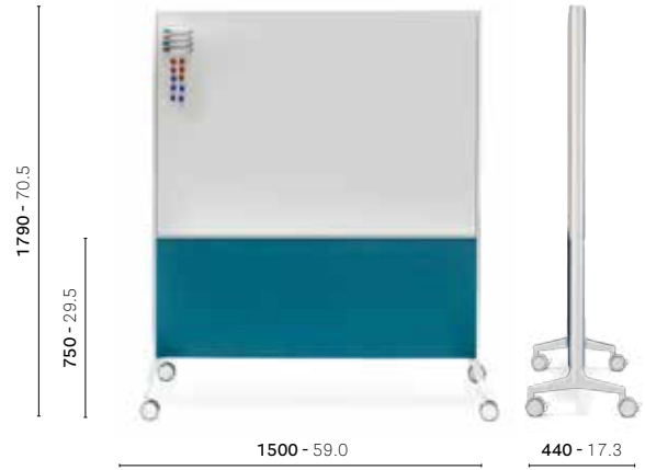
YCL_L150 Space divider with magnetic whiteboard, aluminium structure with castors
