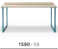
TOA3S_159X150 Desk Table 2 stations, die-cast aluminium legs, solid laminate top, setting for divider panel, single cable management (1300x60 - 51.2x2.4)
